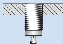
Flush mounting
