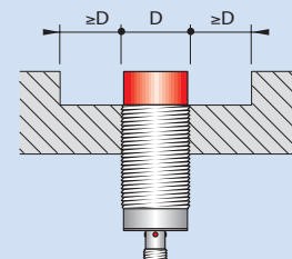
Non flush mounting
