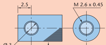
SIDE VIEWER 90° AT-4102
